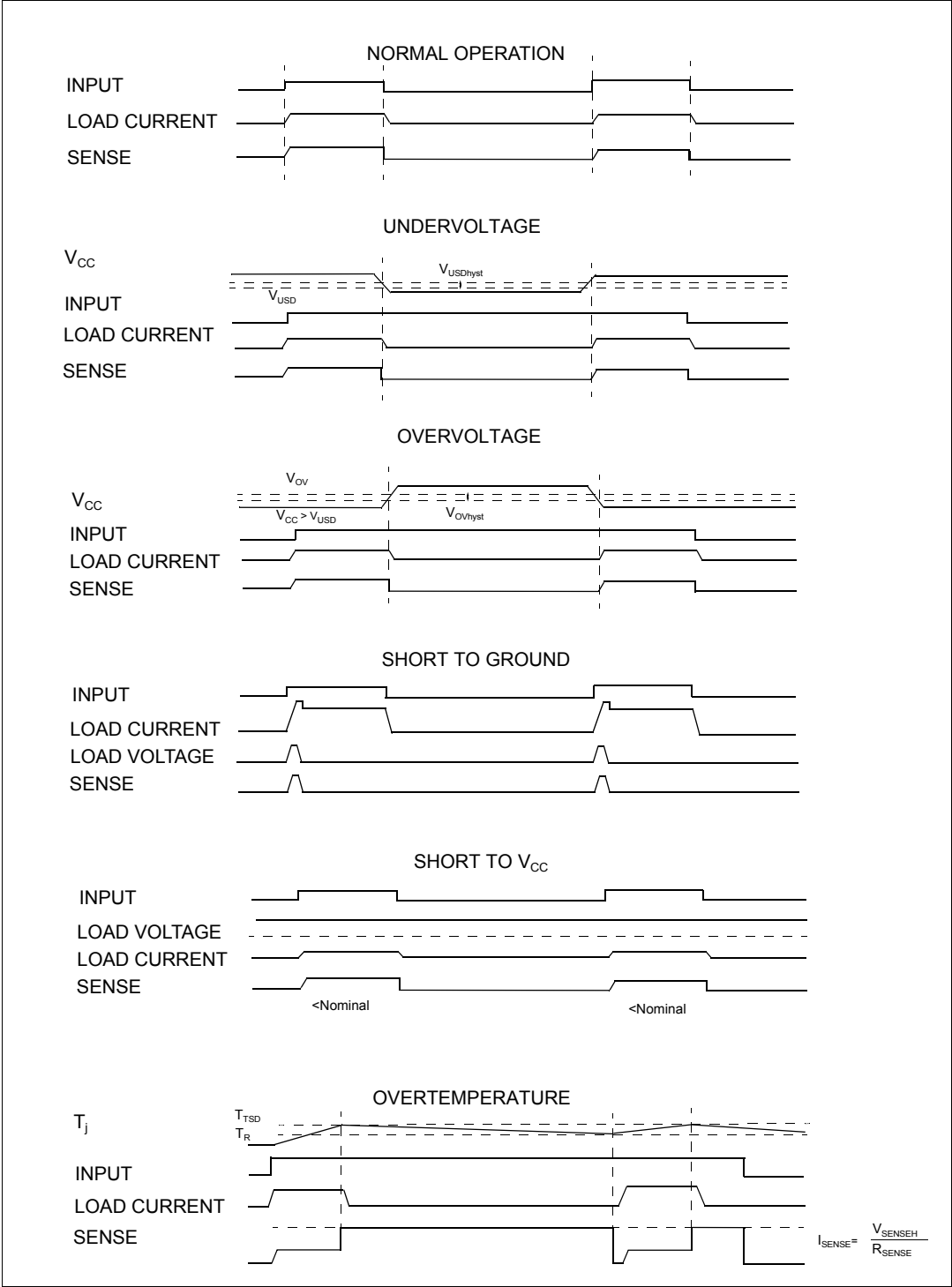
Figure 6. Waveforms
