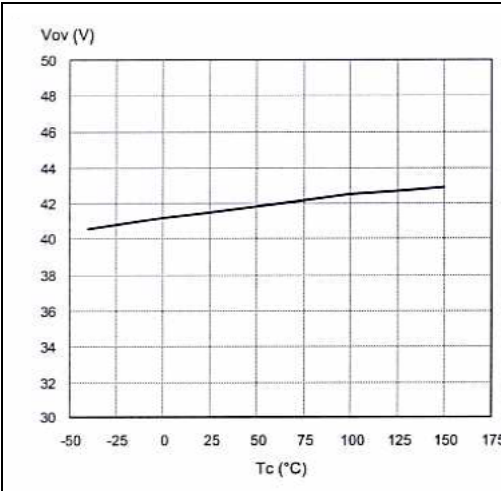
Figure 17. Overvoltage shutdown
