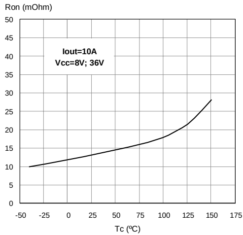
Figure 12. On State Resistance Vs T_{case}
