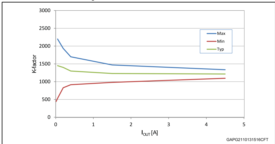
Figure 5: Current sense accuracy versus I OUT
