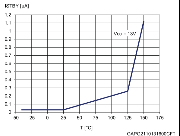
Figure 12: Standby current
