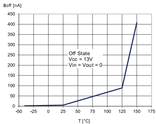
Figure 11: OFF-state output current
