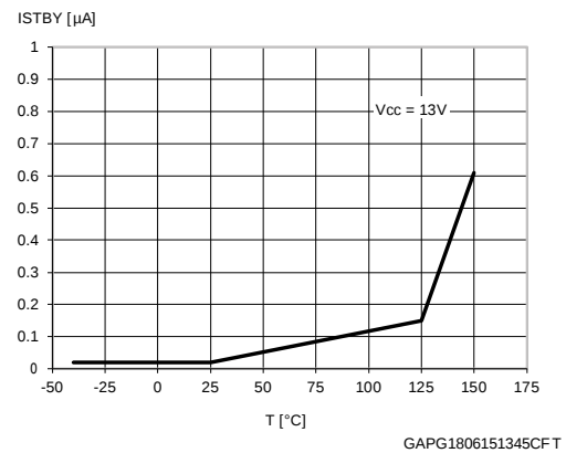
Figure 12: Standby current
