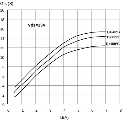
Transconductance
