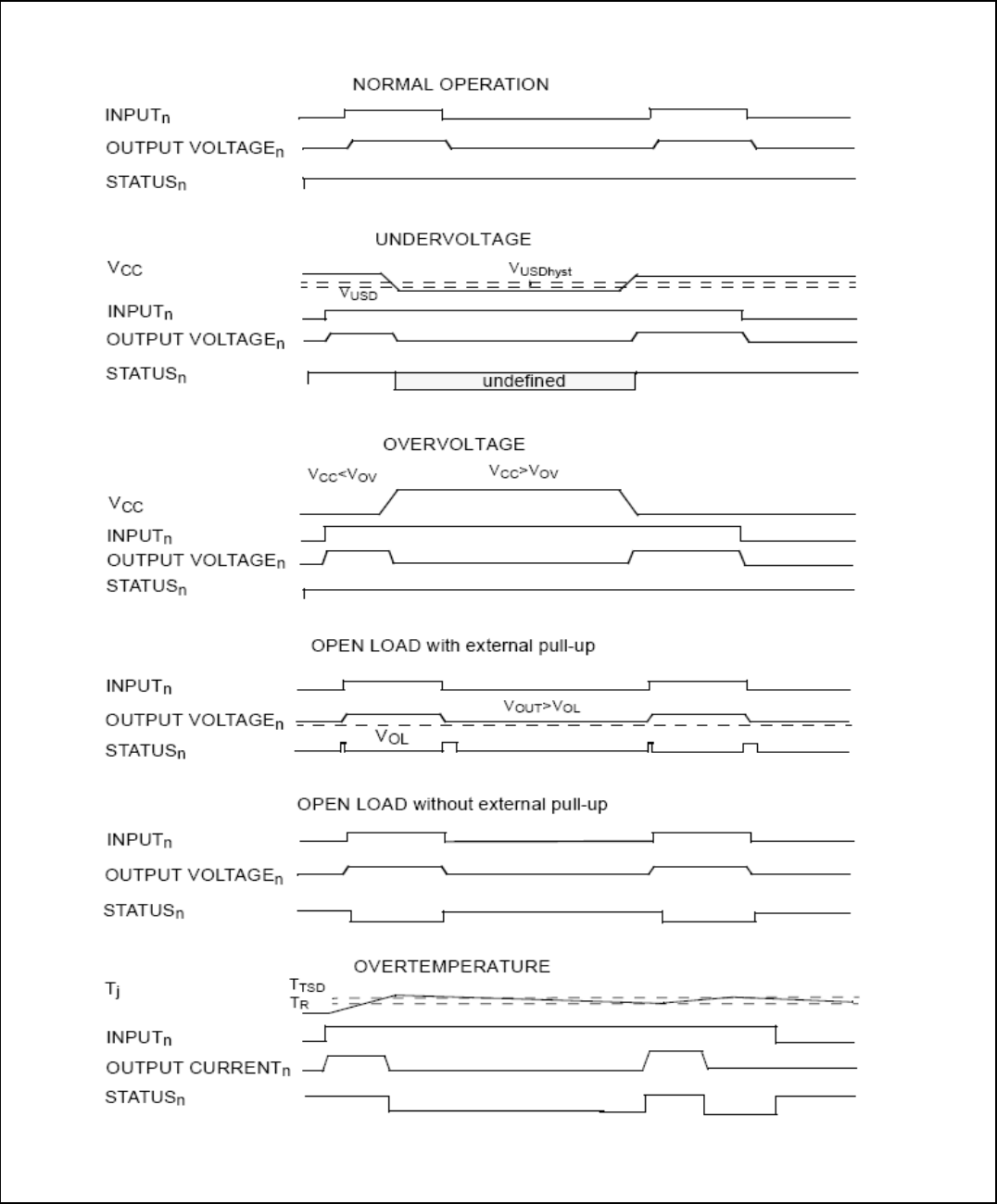
Figure 7. Waveforms
