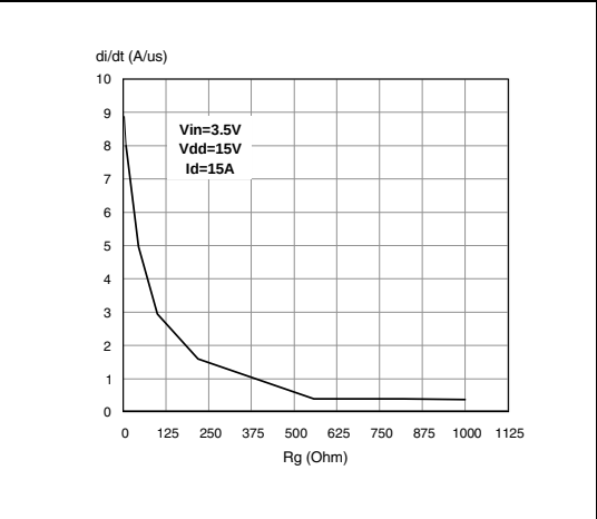
Figure 21. Turn-on current slope, V_{IN} = 3.5 V
