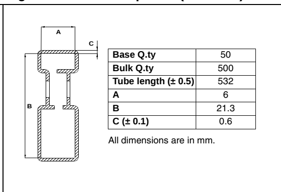
Figure 39. Tube shipment (no suffix)
