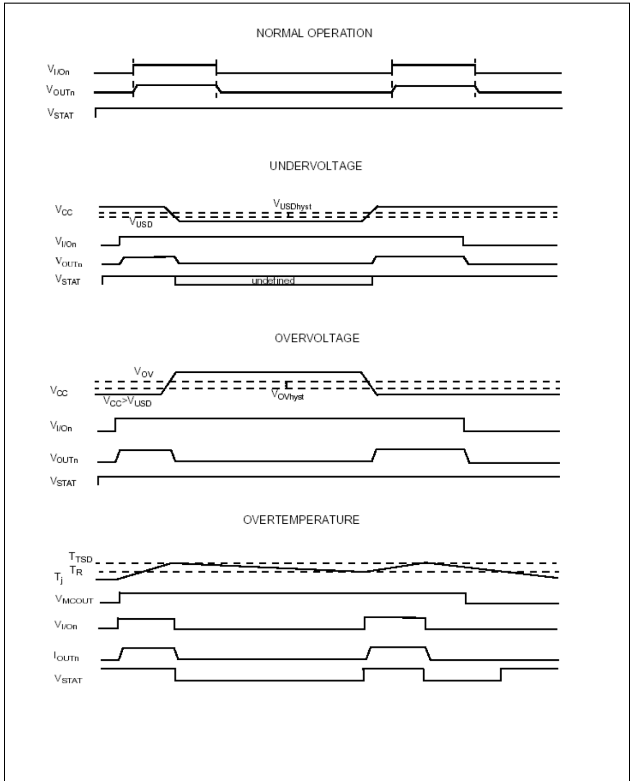
Figure 5. Waveforms
