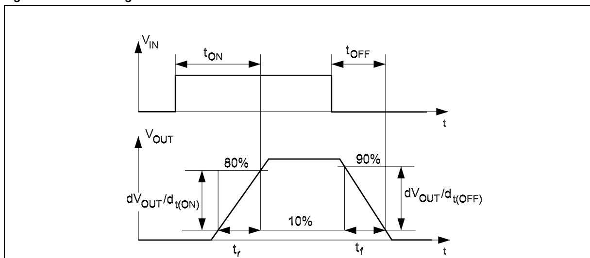
Figure 3. Switching Characteristics
