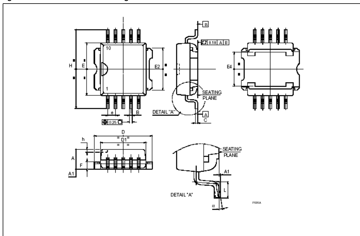
Figure 8. PowerSO-10™ Package Dimensions
