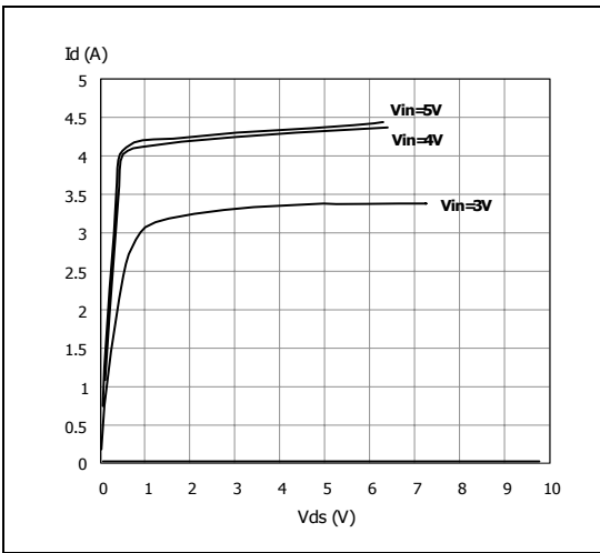
Figure 25. Output characteristics
