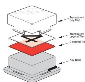
Keypad Assembly
