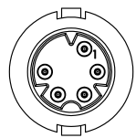
5 POSITION B-KEY #26 PIN & SOCKET CONTACT
