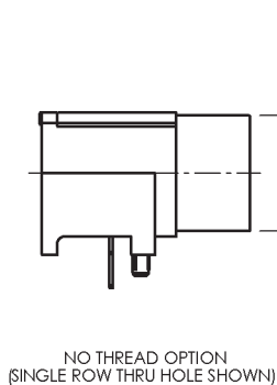
THRU HOLE TERMINATION SINGLE ROW (CONFIG. 3 & 4)
