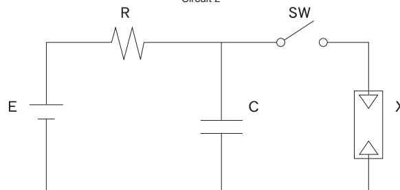
Circuit 2
