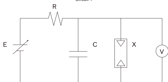
Circuit 1
