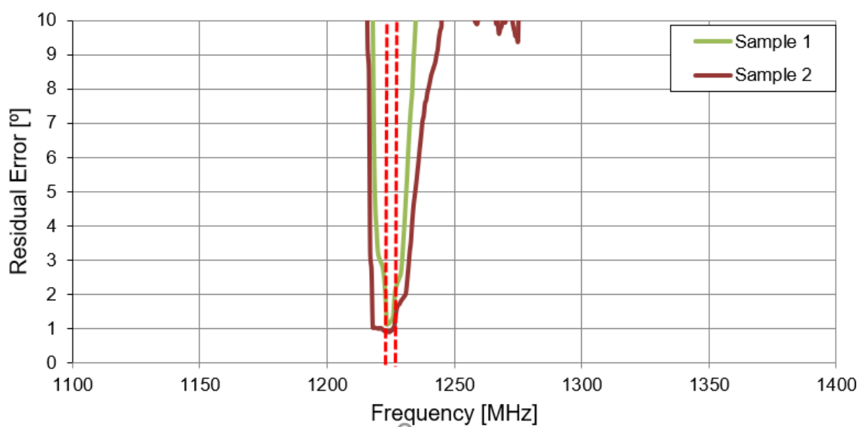
AGPSF.36C.07.0100A L2 Residual Error
