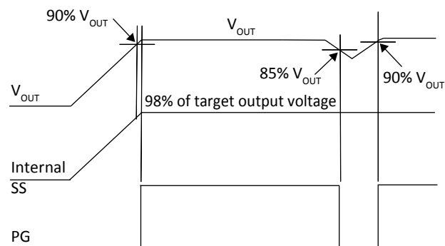
Figure 14 PG signal when PGControl bit=0
