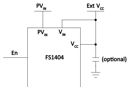
Figure 7 Using an external bias voltage
