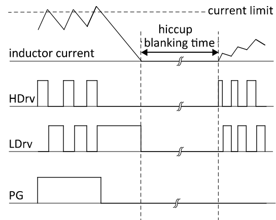
Figure 12 Illustration of OCP in hiccup mode
