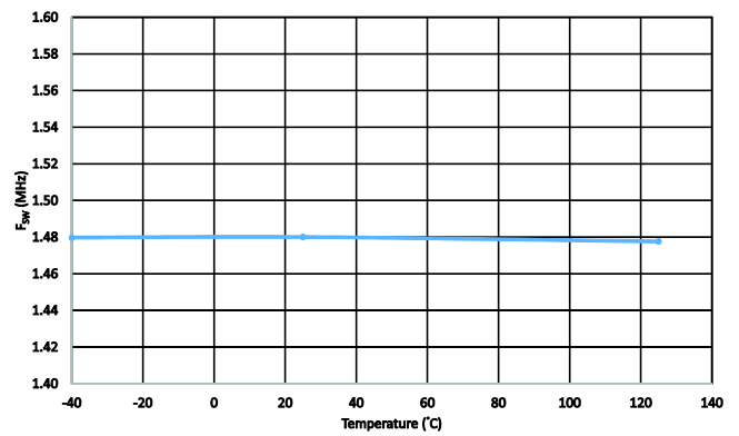
Switching Frequency
