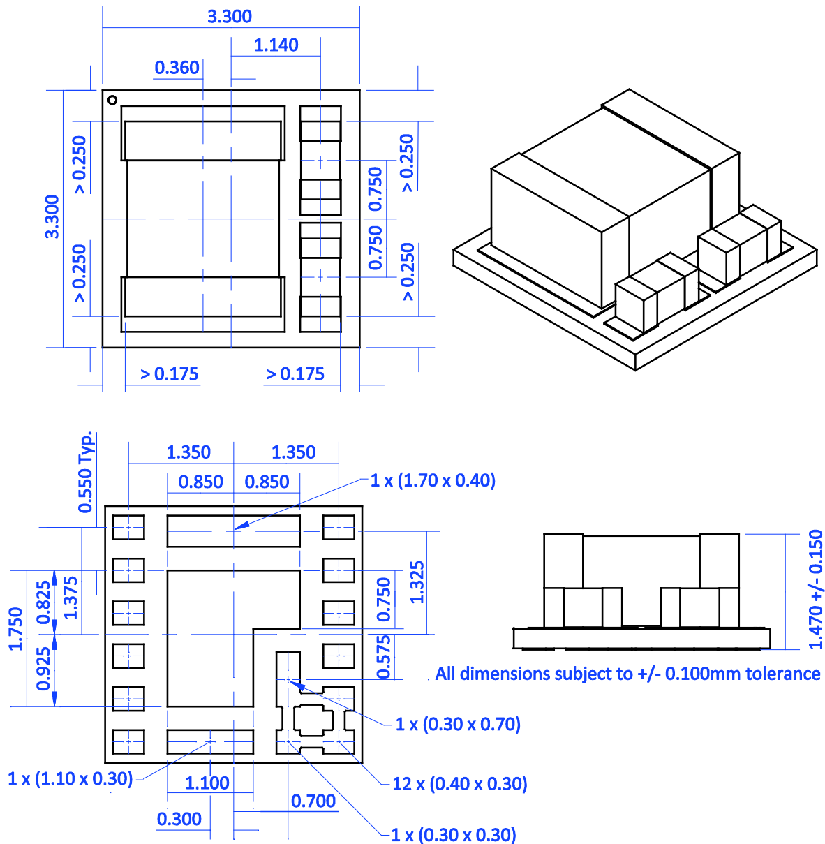
Figure 32 Dimensioned drawings
