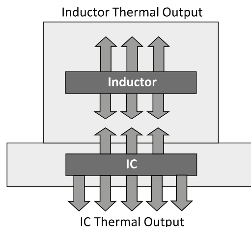
Figure 29 Heat sources in the FS1404
