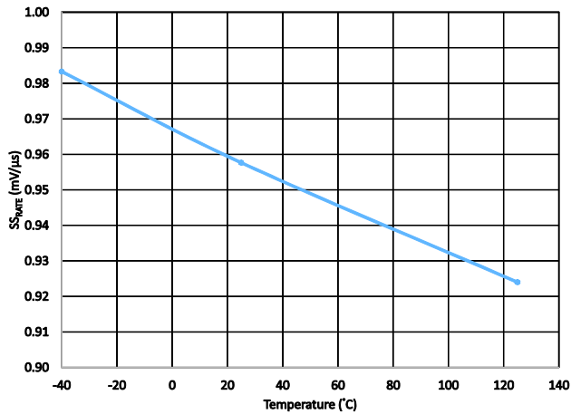
Soft-Start Rate
