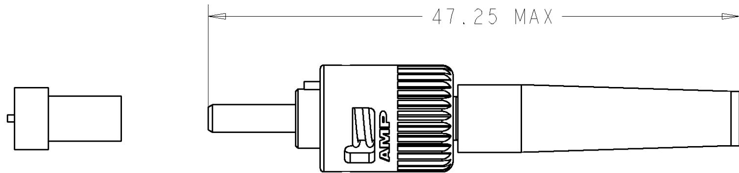
ASSEMBLED CONNECTOR (SHORT BOOT)
