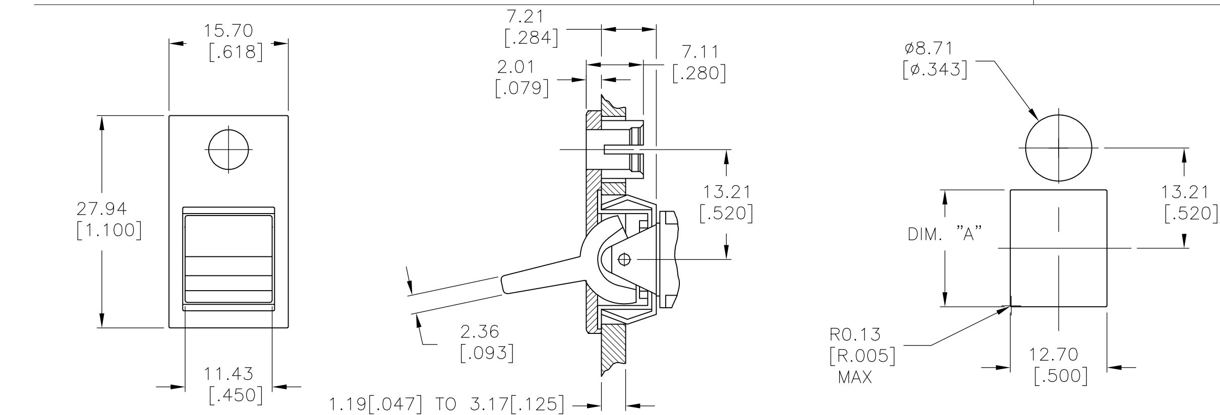
J62 SNAP-IN WITH BEZEL/L.E.D.
