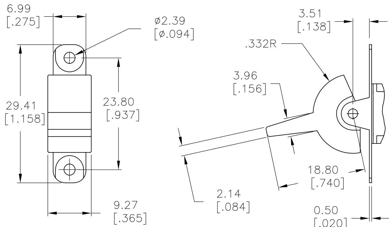
J2 SMALL
