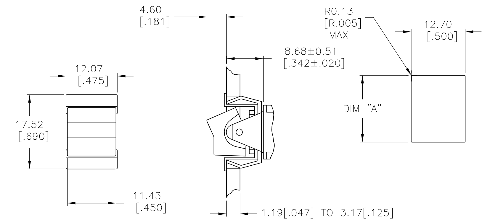
J50 SNAP-IN
