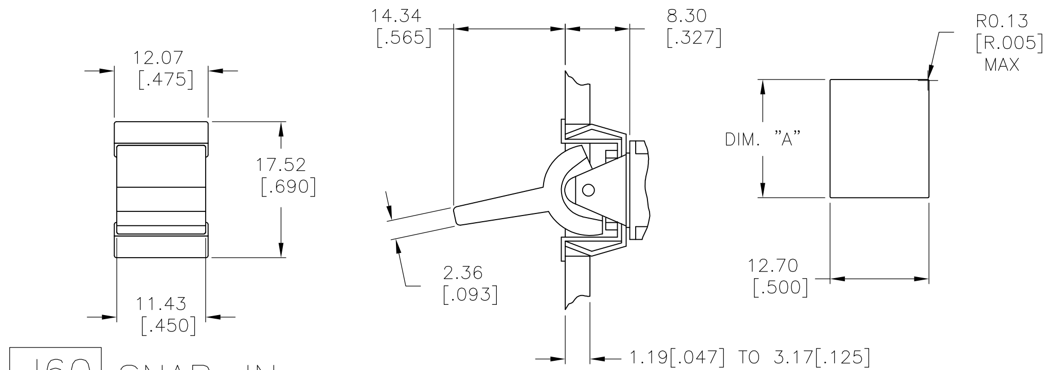
J60 SNAP-IN
