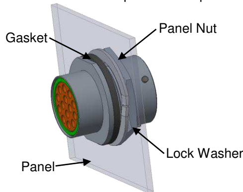
Panel Nut Mounting Torque
