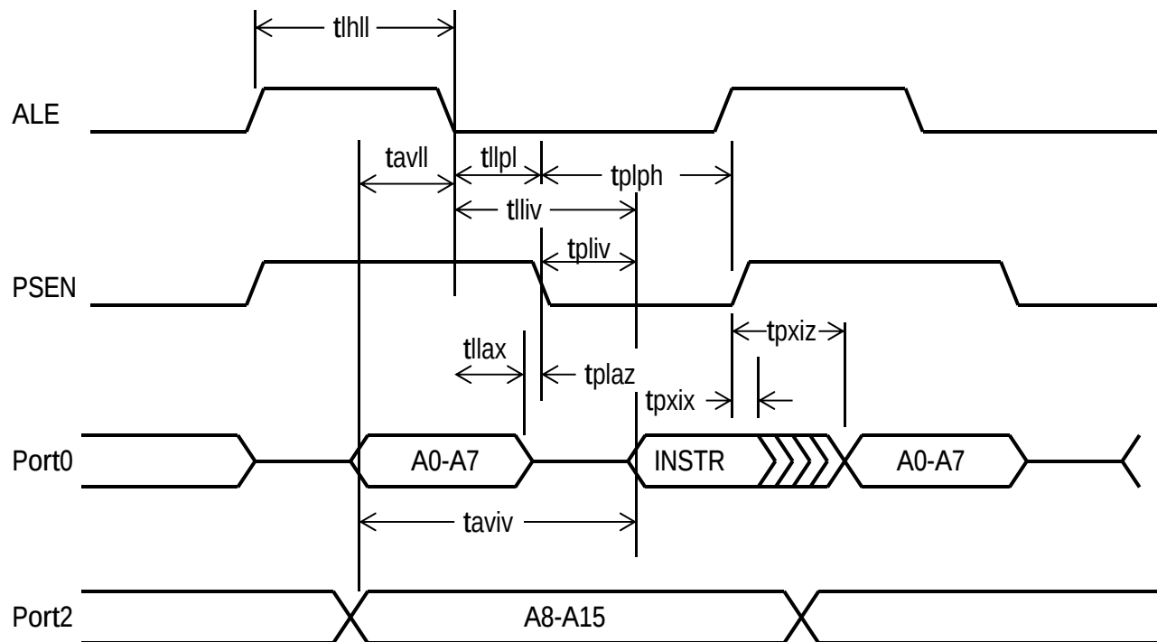
Figure Time-1 – External Program Memory Read Cycle
