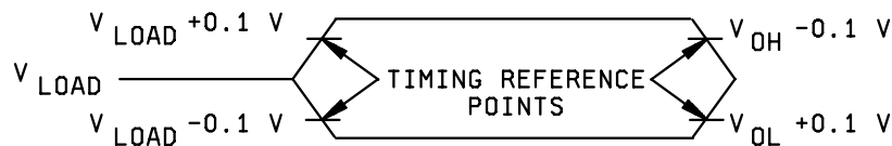
FLOAT WAVEFORM
