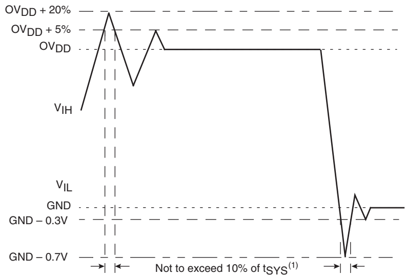
Figure 5-1. Overshoot/Undershoot Voltage
