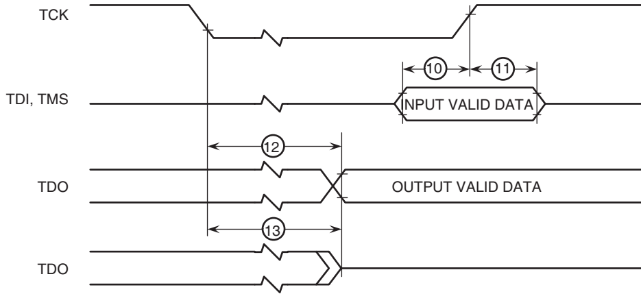
Figure 2-18. Test Access Port Timing Diagram
