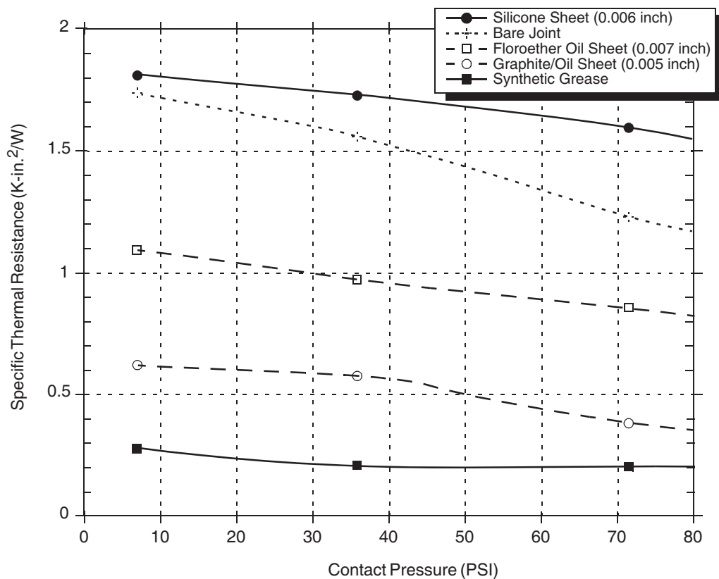
Figure 1-9. Thermal Performance of Select Thermal Interface Material
