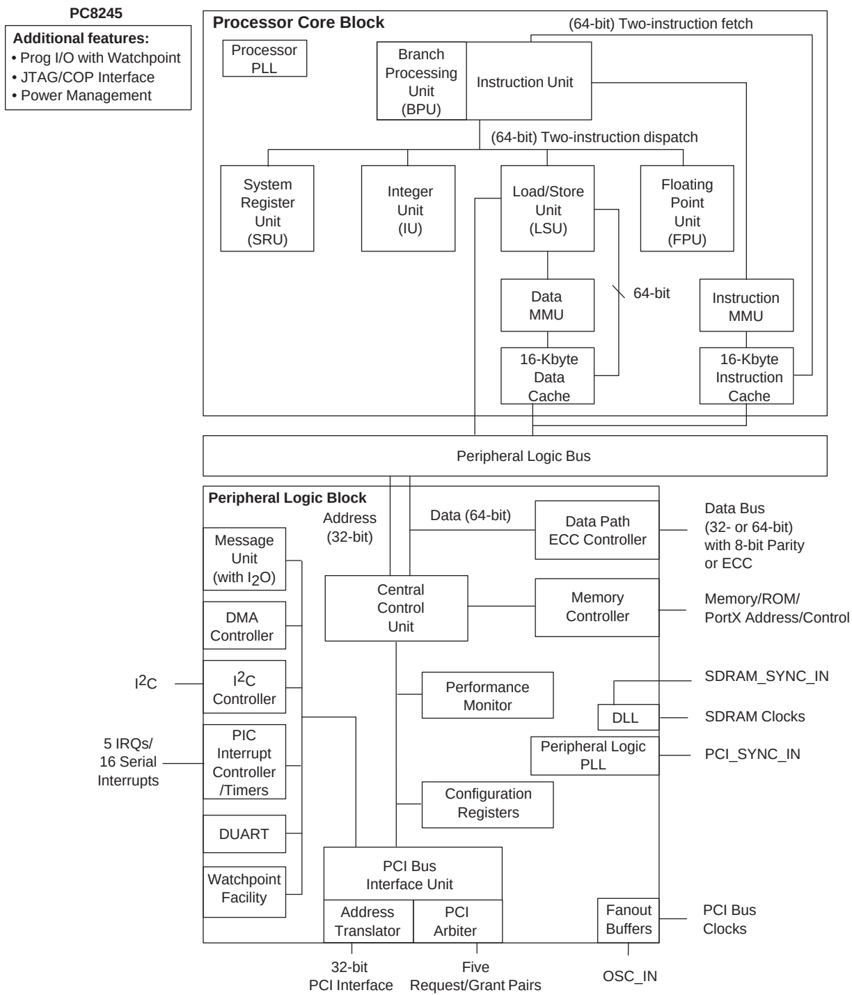
Figure 1-1. Block Diagram
