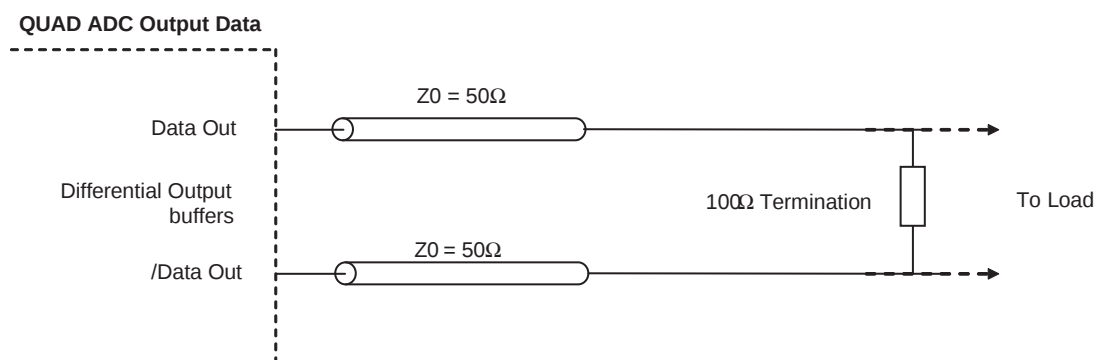
Figure 7-6. Differential Digital Outputs Terminations (100Ω LVDS)
