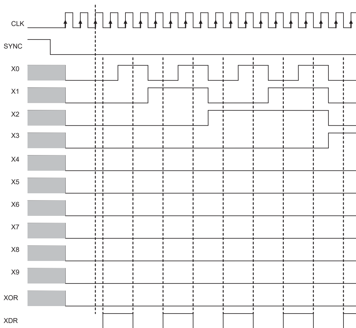
Figure 6-8. Ramp Mode
