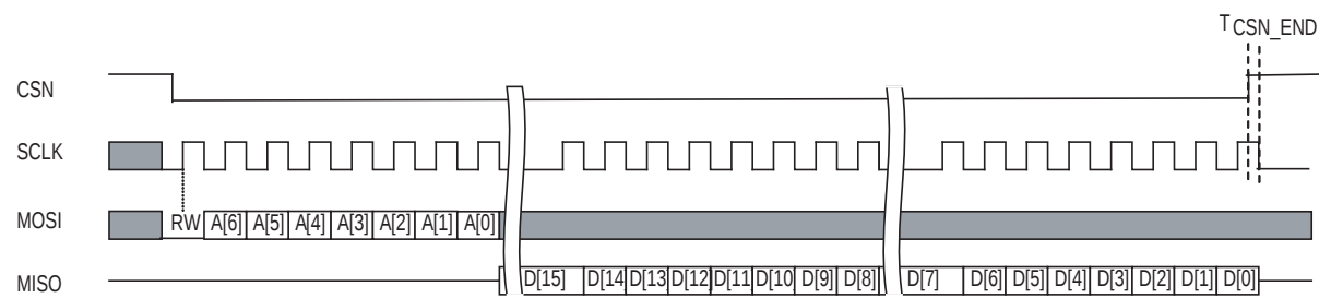
Figure 6-7. Register Read from a 16-bit Register
