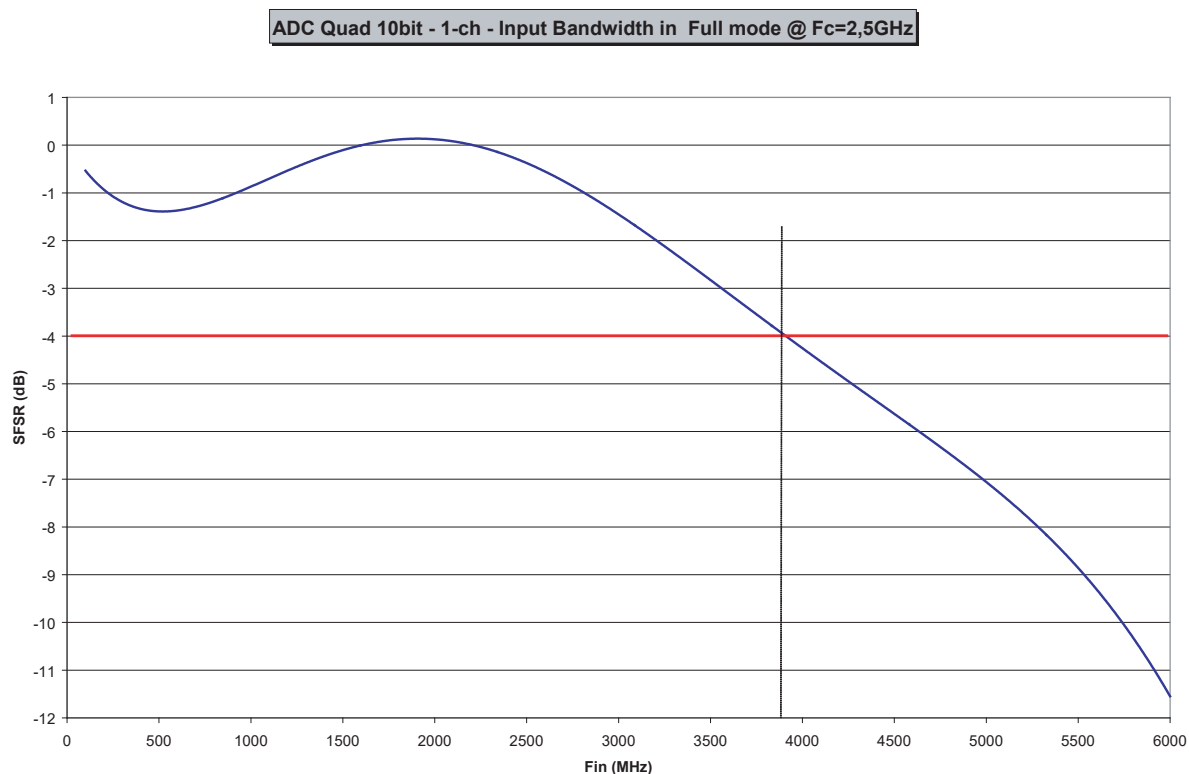
Figure 4-1. Normalized Full Power Input Bandwidth (-1 dBFS Input, 1-channel Mode, F_c = 2.5\text{GHz} , Full Bandwidth Setting)
