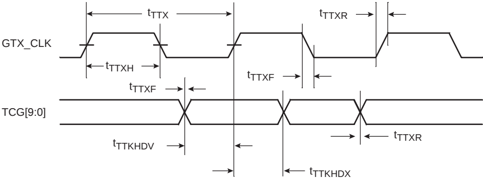
Figure 8-9. TBI Transmit AC Timing Diagram
