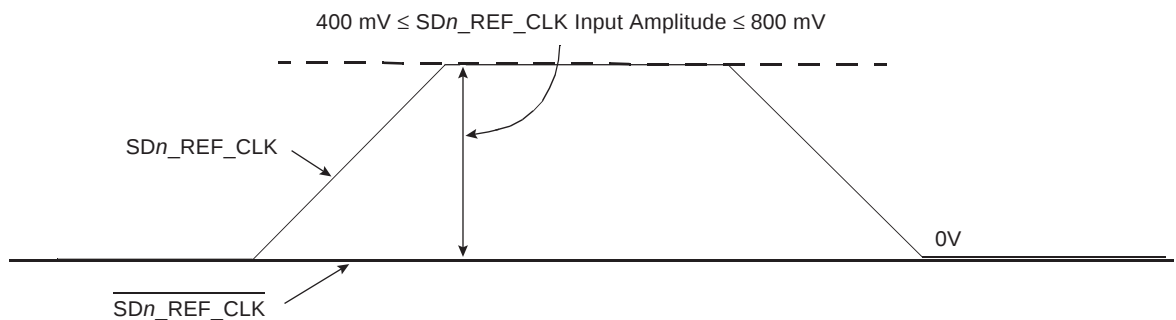
Figure 16-5. Single-Ended Reference Clock Input DC Requirements
