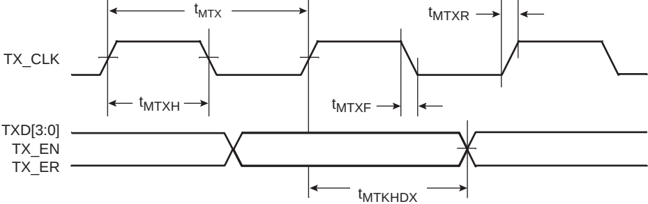
Figure 8-6. MII Transmit AC Timing Diagram
