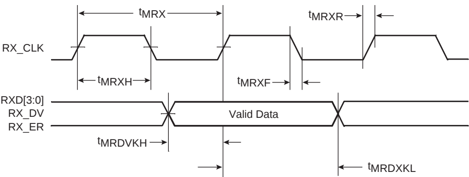
Figure 8-8. MII Receive AC Timing Diagram
