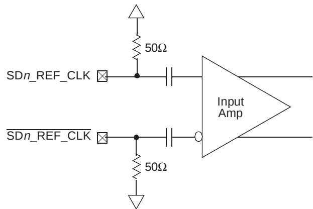
Figure 16-2. Receiver of SerDes Reference Clocks
