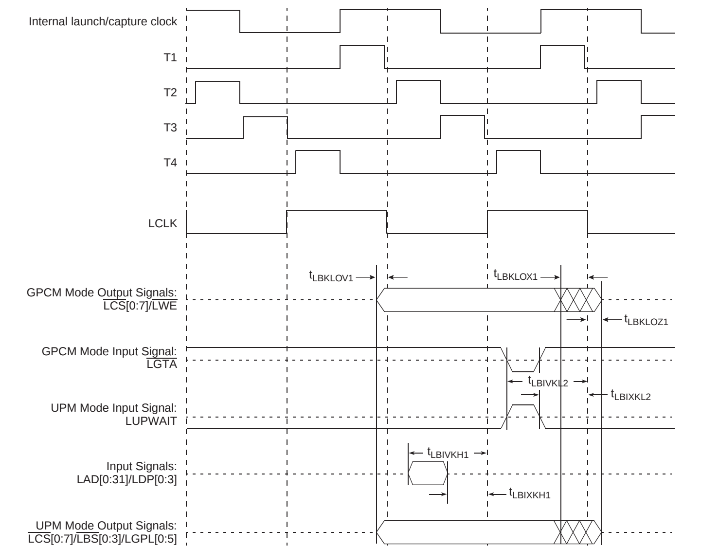
Figure 10-7. Local Bus Signals, GPCM/UPM Signals for LCCR[CLKDIV] = 8 or 16 (PLL Bypass Mode)
