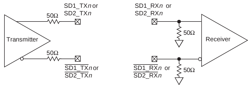
Figure 16-10. SerDes Transmitter and Receiver Reference Circuits
