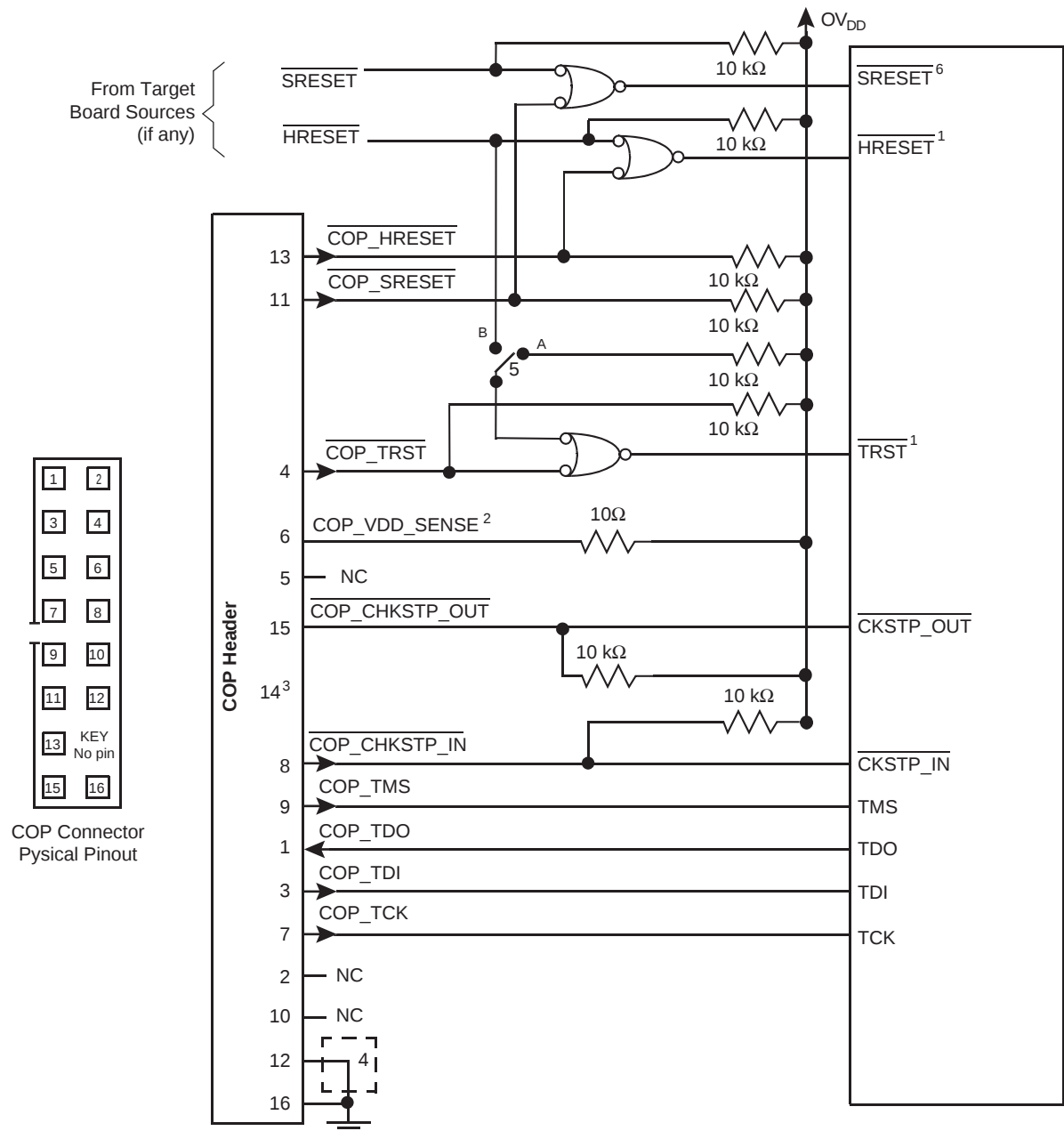
Figure 22-7. JTAG Interface Connection
