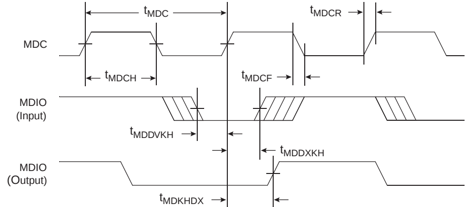
Figure 9-1. MII Management Interface Timing Diagram
