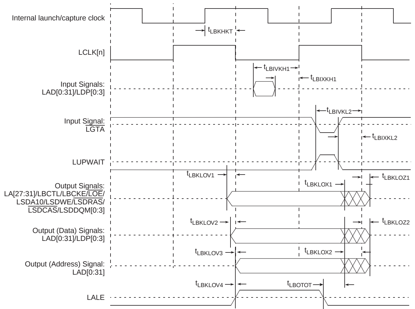
Figure 10-3. Local Bus Signals (PLL Bypass Mode)
