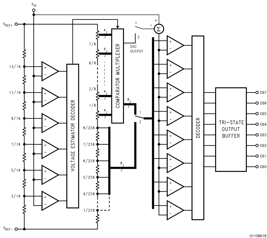
FIGURE 6. Block Diagram of the ADC08061/2 Multi-Step Flash Architecture
