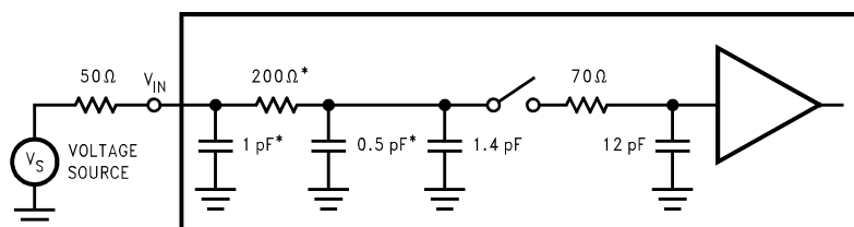
FIGURE 7. ADC08061 and ADC08062 Equivalent Input Circuit Model
