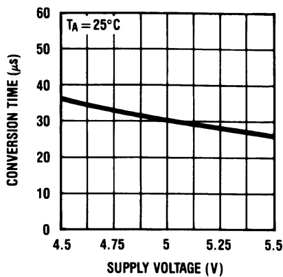
Conversion Time vs. V SUPPLY
