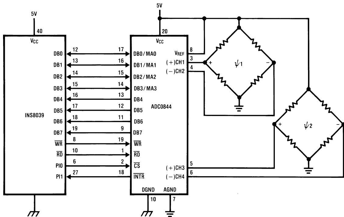
ADC0844—INS8039 Interface
