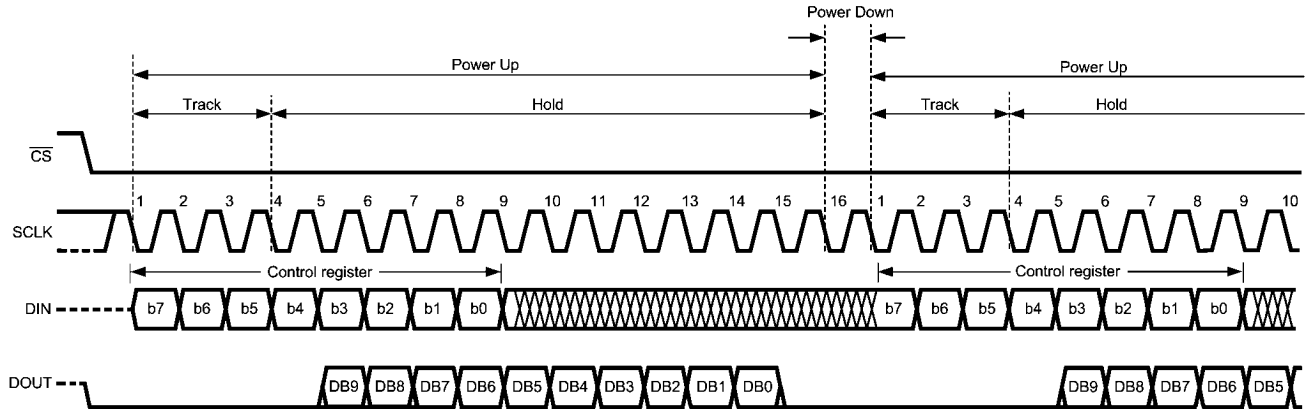
ADC102S051 Operational Timing Diagram
