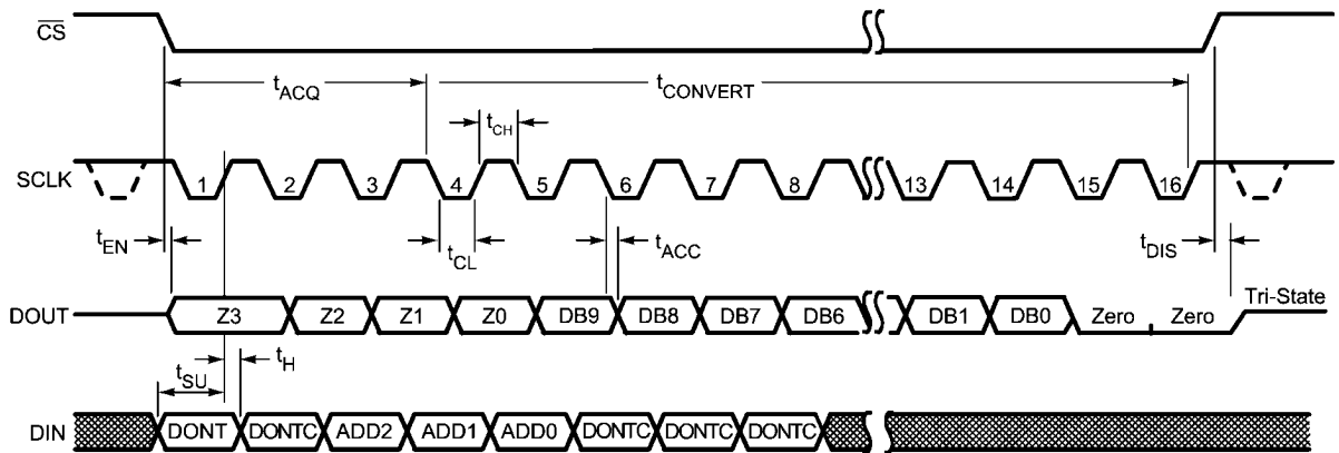
ADC102S051 Serial Timing Diagram
