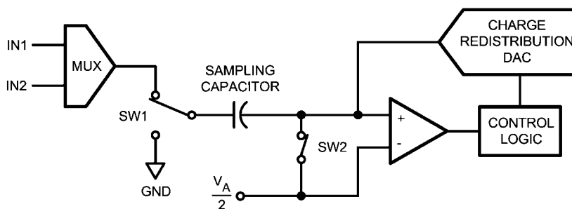
FIGURE 1. ADC102S051 in Track Mode
