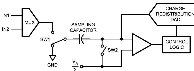
FIGURE 2. ADC102S051 in Hold Mode
