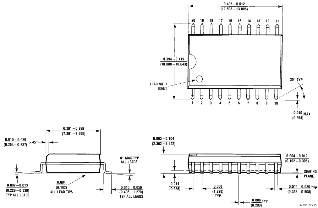
Order Number ADC10461CIWM NS Package Number M20B
