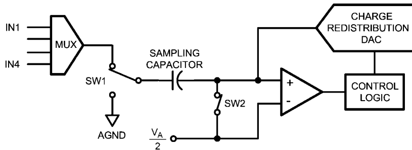
FIGURE 1. ADC104S101 in Track Mode
