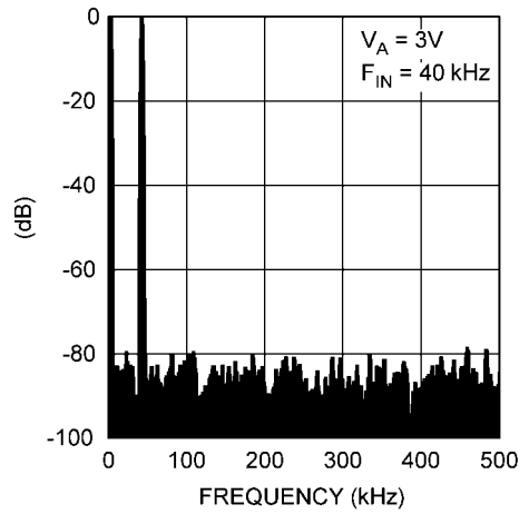
Spectral Response - 3V, 1.0 Mpsps
