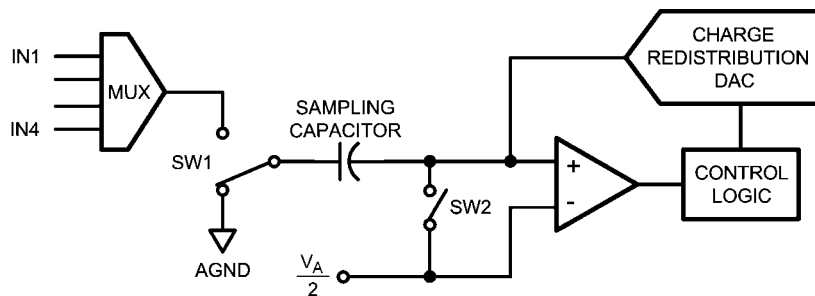
FIGURE 2. ADC104S101 in Hold Mode
