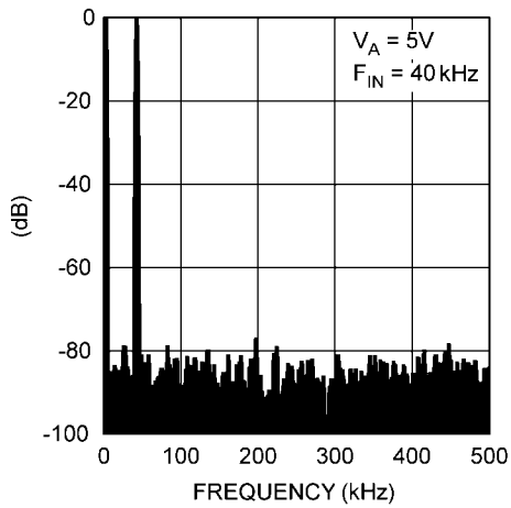
Spectral Response - 5V, 1.0 Mpsps
