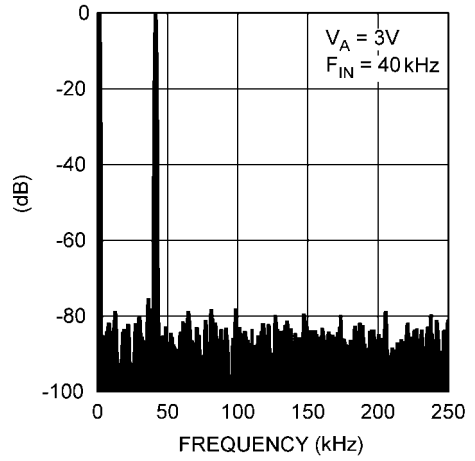
Spectral Response - 3V, 500 kpsps
