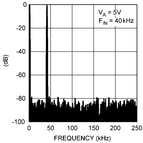
Spectral Response - 5V, 500 kpsps
