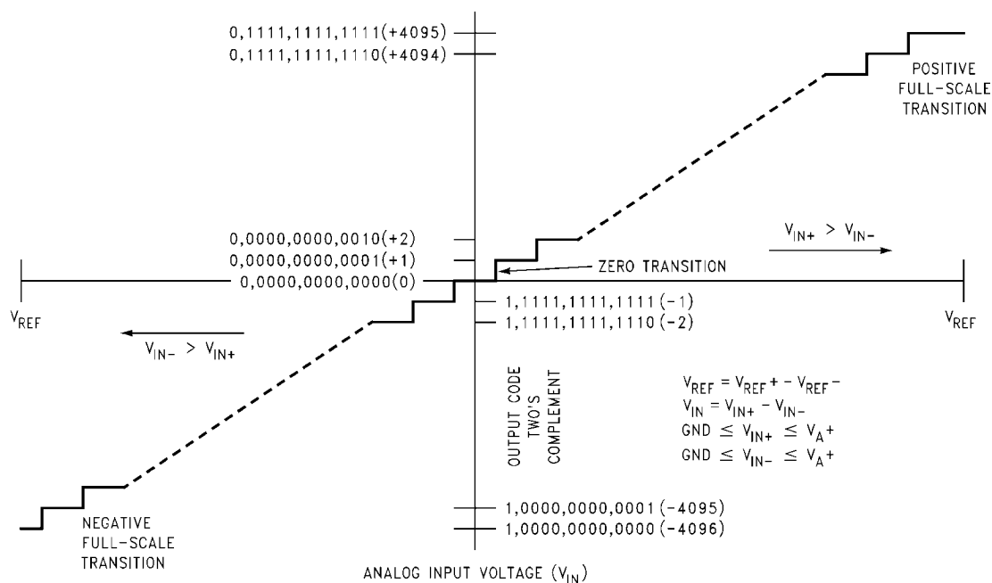
FIGURE 1. Transfer Characteristic
