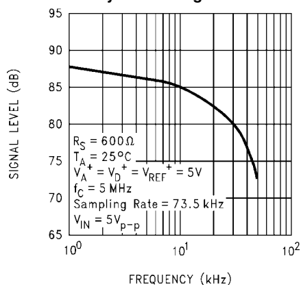
Bipolar Spurios Free Dynamic Range
