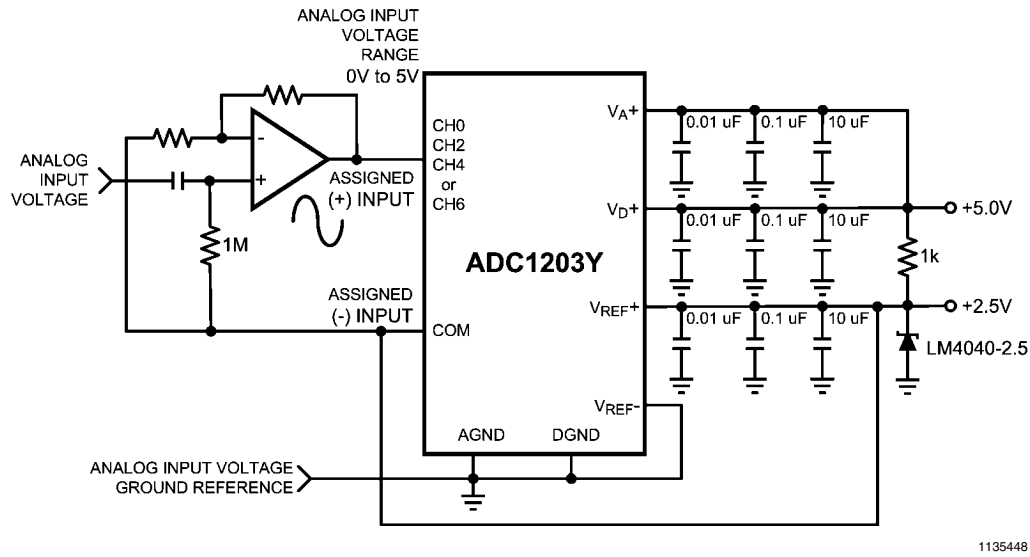
FIGURE 13. Alternative Pseudo-Differential Biasing
