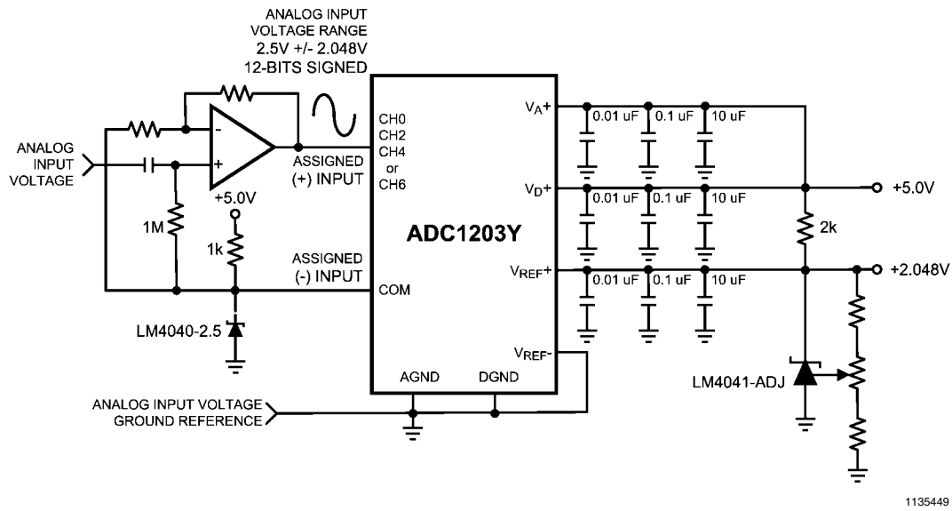
FIGURE 14. Pseudo-Differential Biasing without the Loss of Digital Output Range
