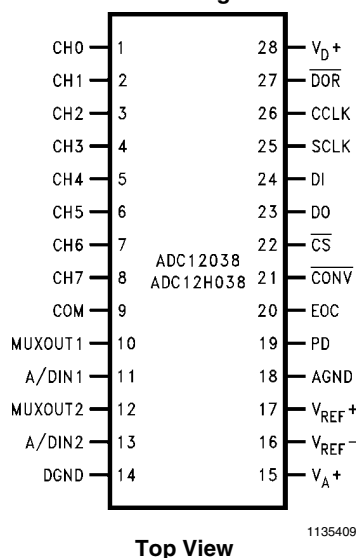
28-Pin Wide Body SO Packages
