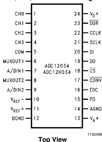
24-Pin Wide Body SO, DIP, SSOP-EIAJ Packages
