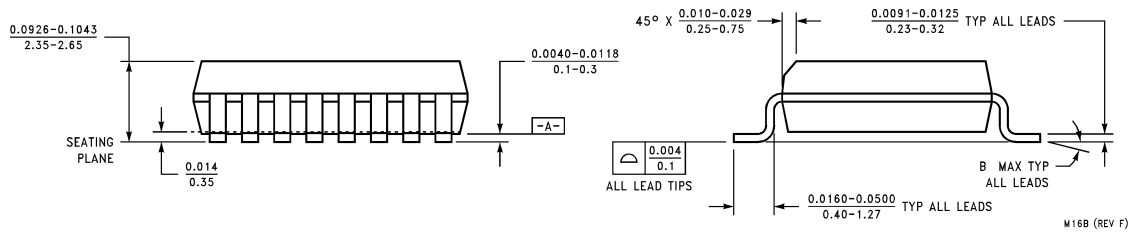
Order Number ADC12130CIWM NS Package Number M16B
