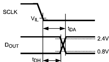
FIGURE 5. D OUT Hold and Access Times
