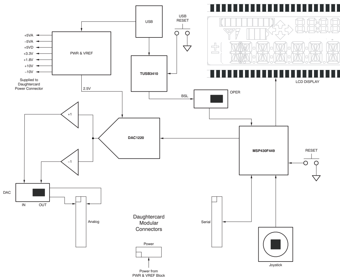
Figure 8. MMB3 Block Diagram
