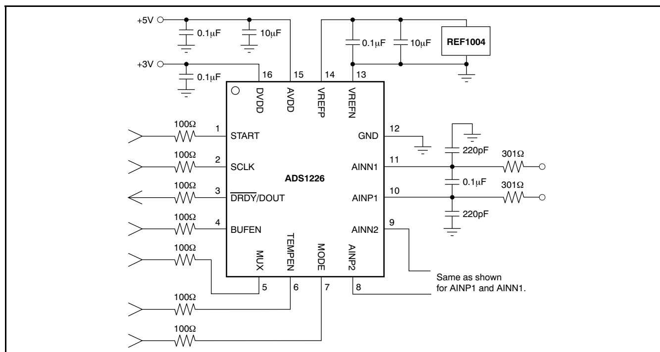
Figure 31. Basic Connections
