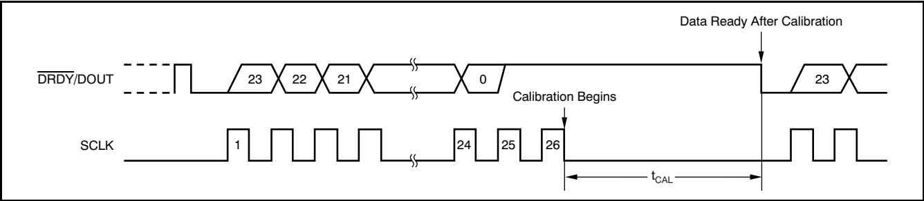
Figure 30. Self-Calibration Timing
