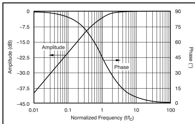
Figure 34. HPF Amplitude and Phase Response
