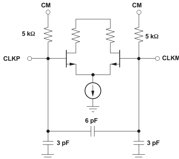
Figure 45. Clock Inputs
