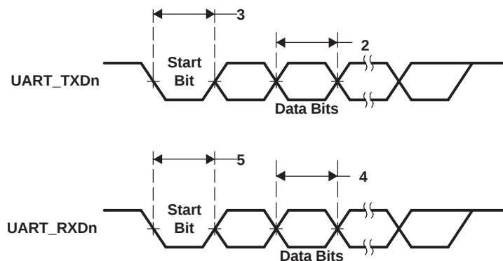
Figure 5-42. UART Transmit/Receive Timing
