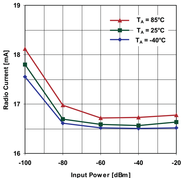
1.2 kBaud GFSK
