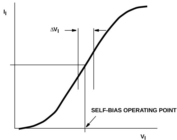
FIGURE 12. TYPICAL INPUT RESISTANCE CURVE AT SIG IN , COMPI IN
