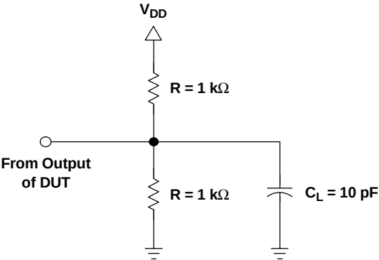
Figure 1. LVC MOS Output Test Load
