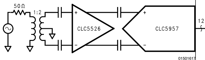
FIGURE 2. Differential I/O Connections
