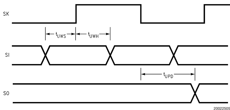
FIGURE 1. MICROWIRE/PLUS Timing
