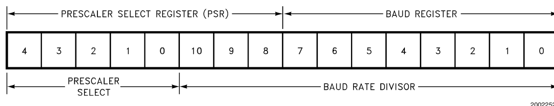
FIGURE 25. USART BAUD Clock Divisor Registers
