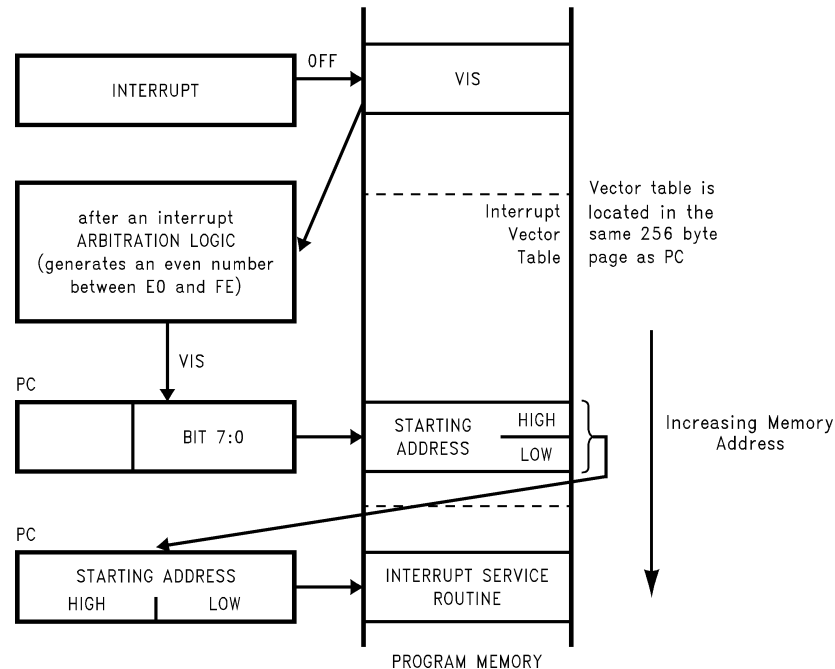
Figure 5-24. VIS Operation
