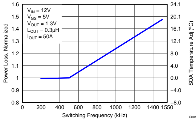
Figure 6. Normalized Power Loss vs Switching Frequency
