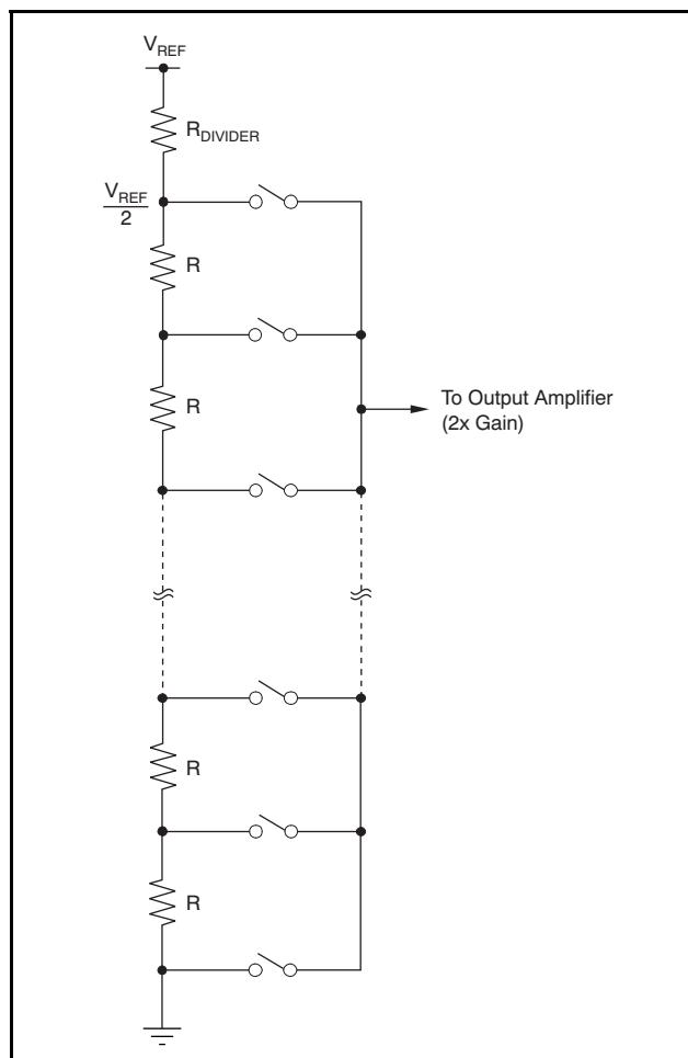
Figure 63. Resistor String
