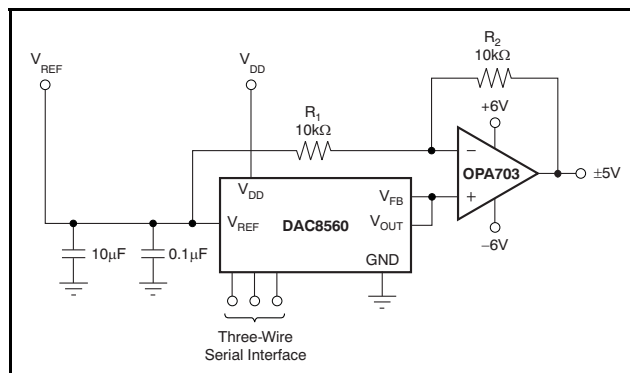
Figure 69. Bipolar Output Range Using External Reference at 5V
