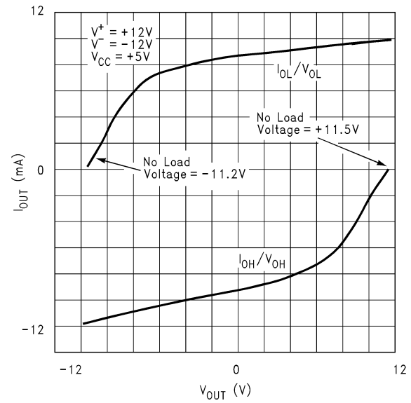
Driver Output Current vs Output Voltage
